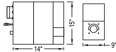
BURNER DIMENSIONS
