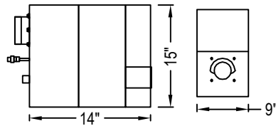
BURNER DIMENSIONS
